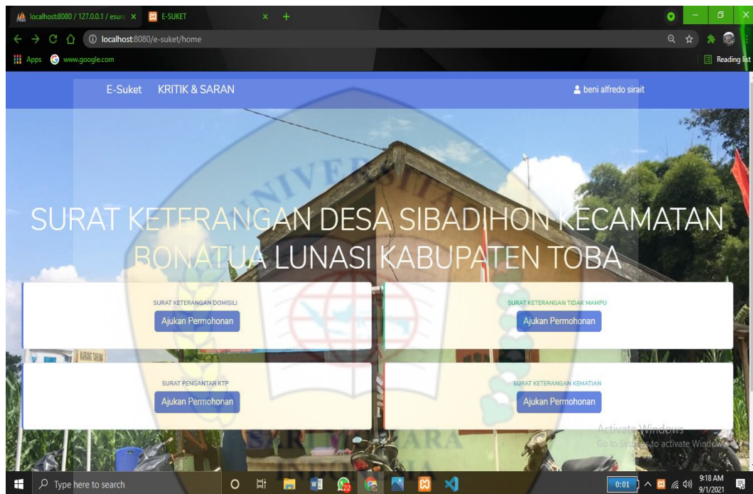
Halaman home
