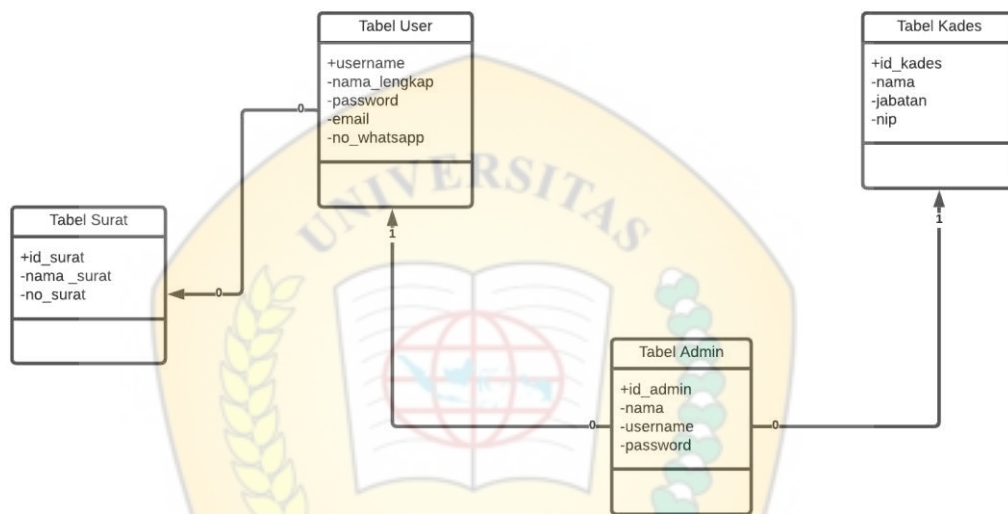
Gambar 3.5 Class Diagram Sistem Pelayanan Mandiri
